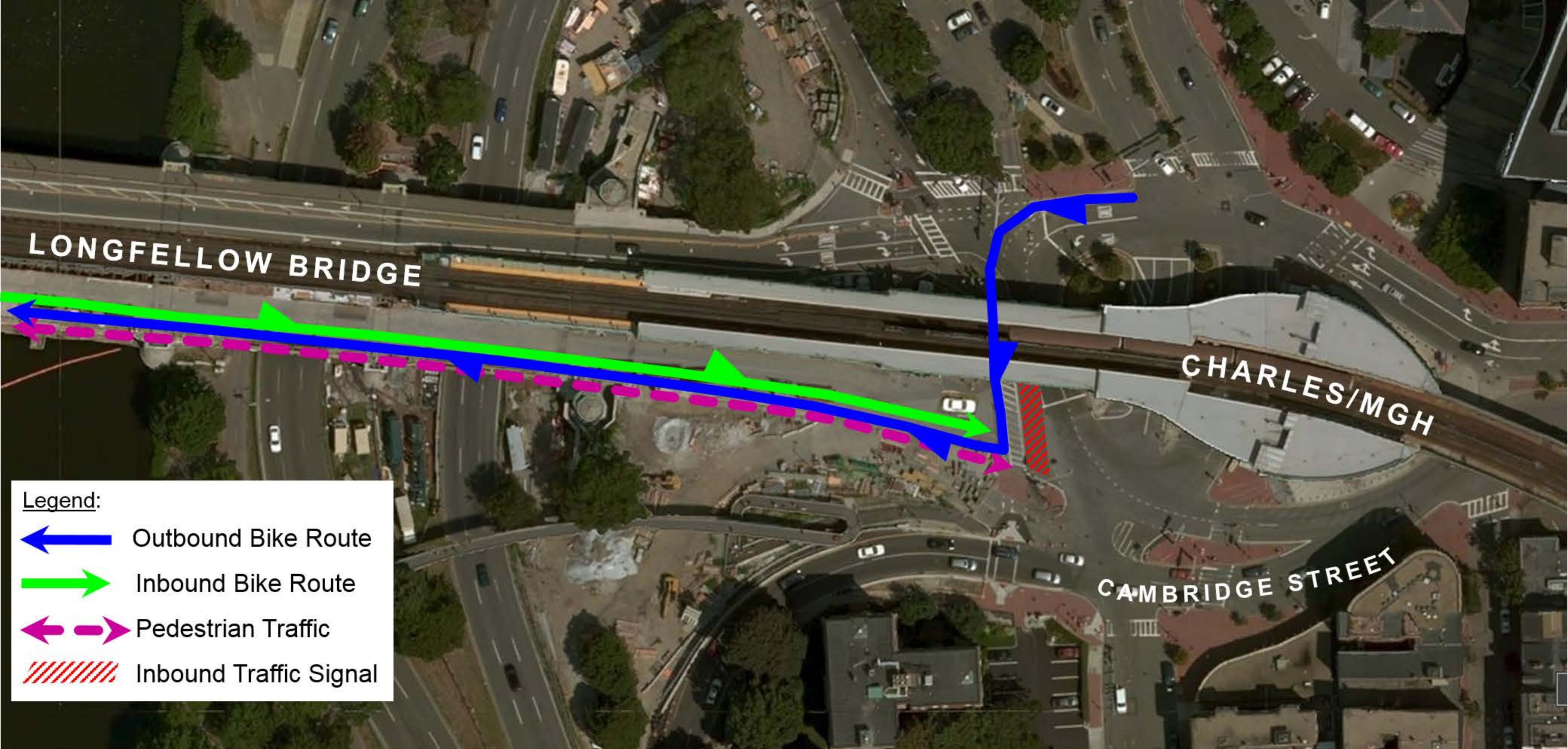
Longfellow Bridge Rehabilitation Project STAGE 4 & 6 Bike and Pedestrian Traffic – Boston Approach
